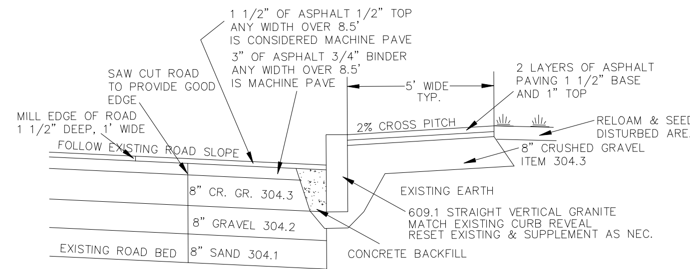
TYPICAL ROAD WIDENING CROSS SECTION
